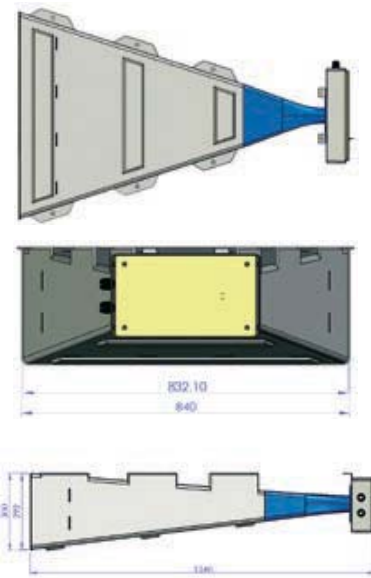
Mechanical drawing with 8 x 12 mm fixation holes and vertical-ribs for extra stability
